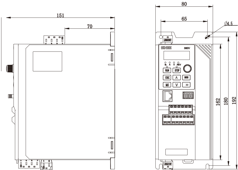
(b) E700-1R5-2B-G~EM700-2R2-2B-G/EM700-2R2-3B-G~EM700-4R0-3B-G Size
