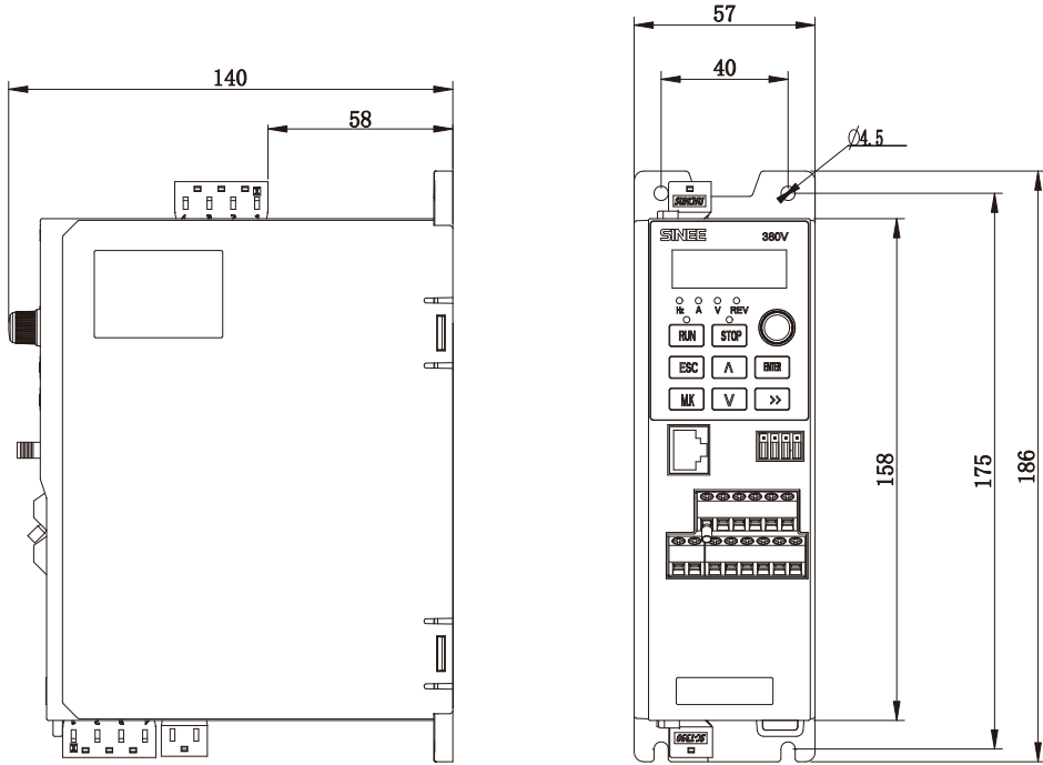
(a) E700-0R4-2B-G~EM700-0R7-2B-G/EM700-0R7-3B-G~EM700-1R5-3B-G Size
